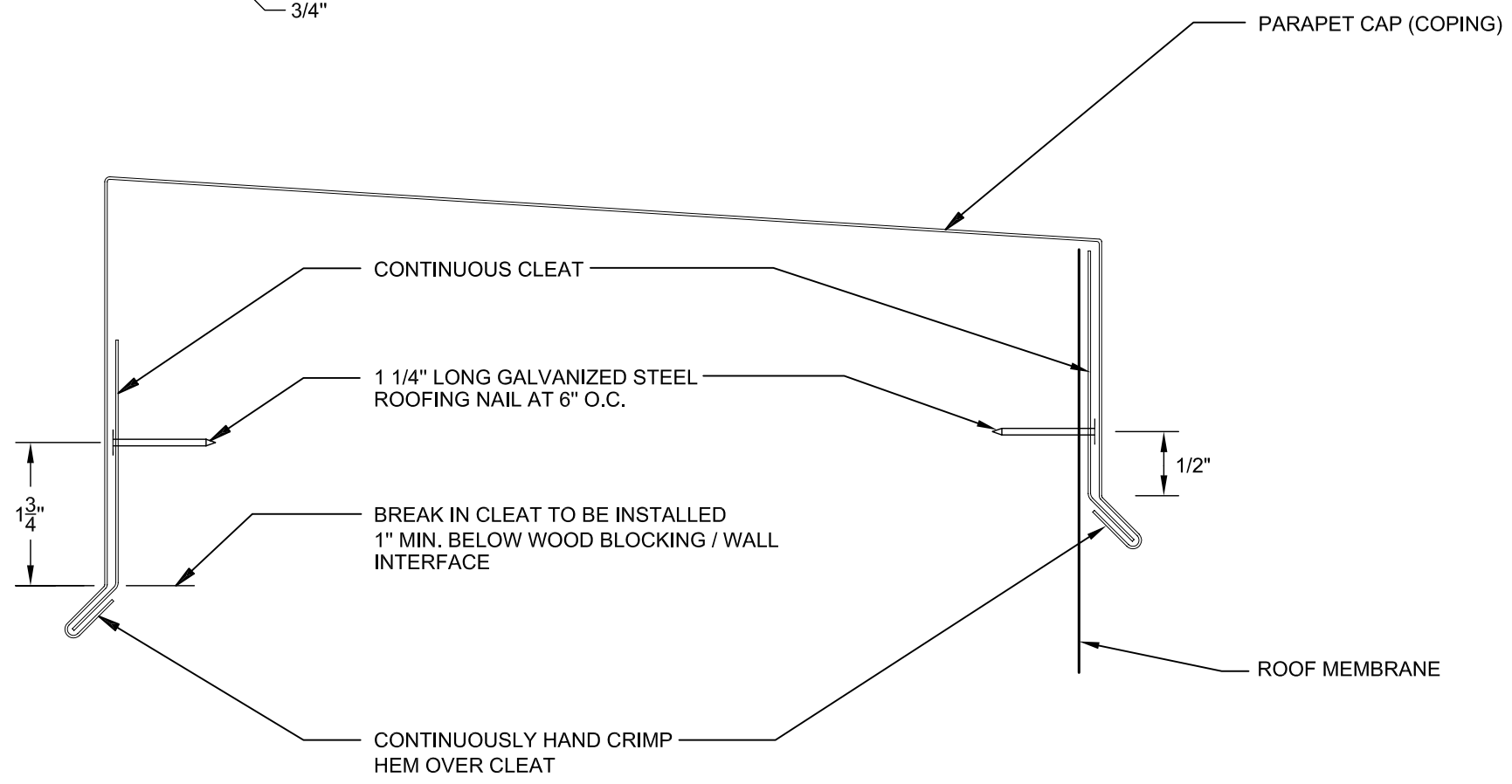
INSTALLATION DRAWING
