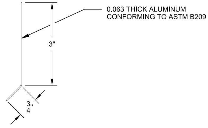
CLEAT
