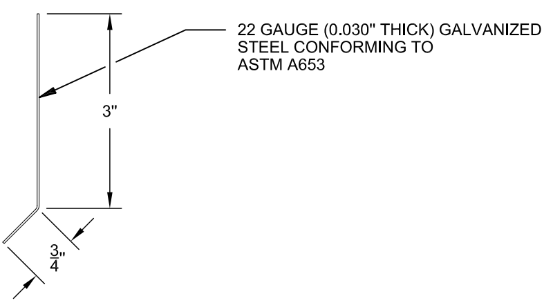
CLEAT
