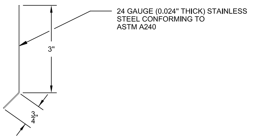
CLEAT
