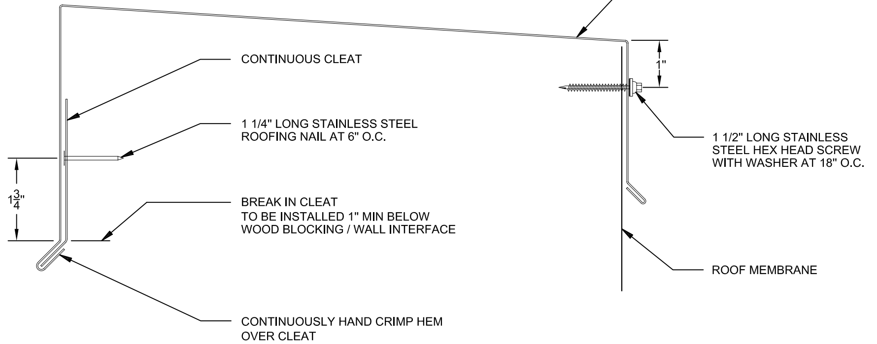
INSTALLATION DRAWING
