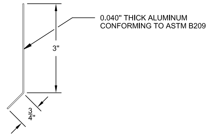
CLEAT
